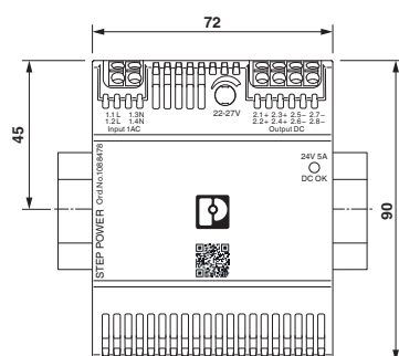
Dimensional drawing
