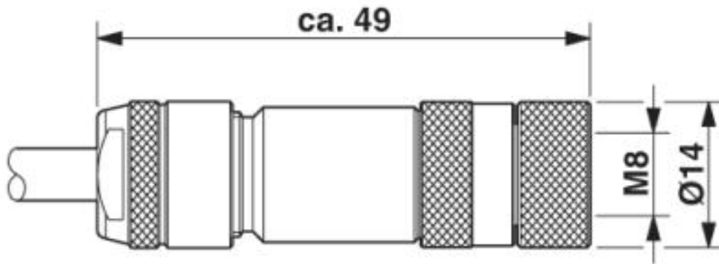
Socket M8 x 1, straight, shielded
