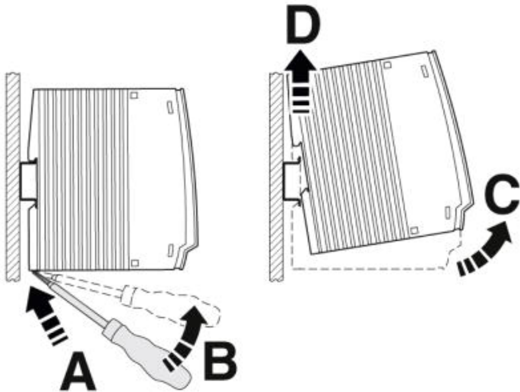
Schematic diagram
